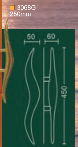
Front view Side view
