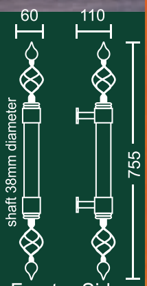
Front view Side view
