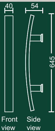
□ 3150S 450mm (width 30mm) back to back set only
